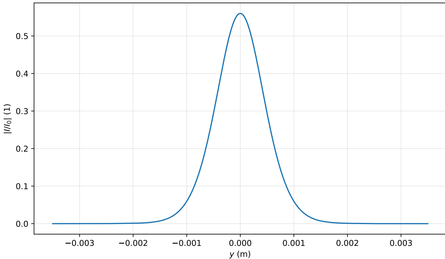
Intensity profile I(x=0, y, z=3.025)/I_0 , P_{in}=0.5P_{cr} , artificial time
